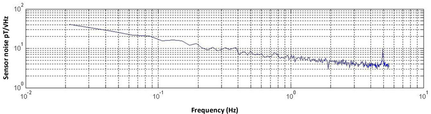
Noise density spectrum of the LEMI-024 Fluxgate Magnetometer
